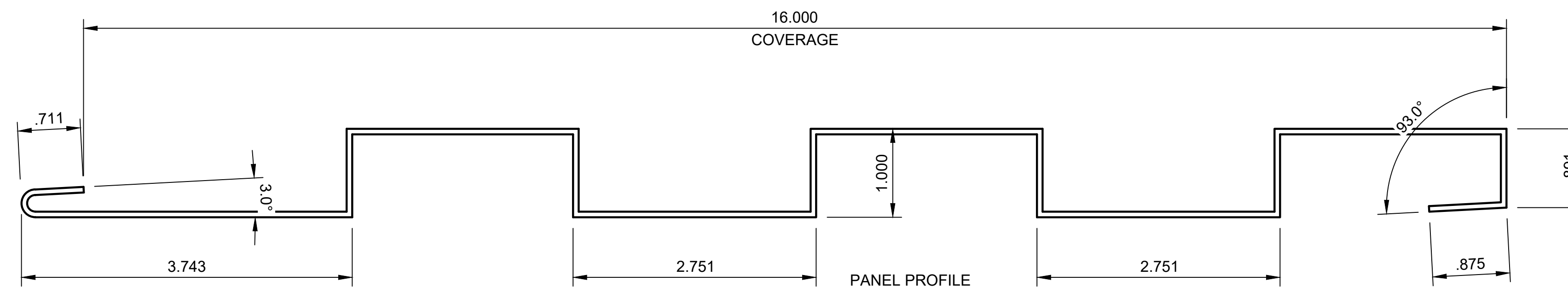
PANEL PROFILE PART# 8300-1 QTY: 10'-0" STOCK LENGTHS
